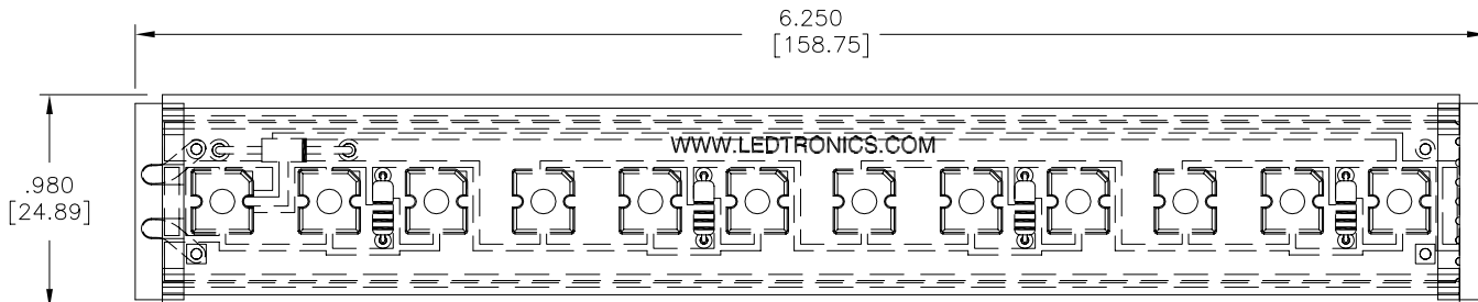
TOP VIEW
