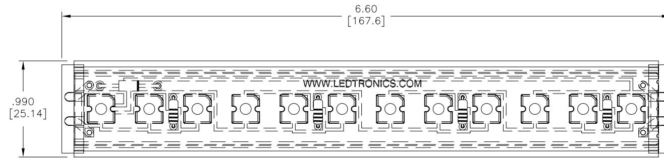
TOP VIEW
