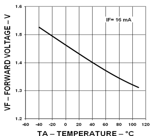
Figure 8: Forward Voltage vs. Temperature
