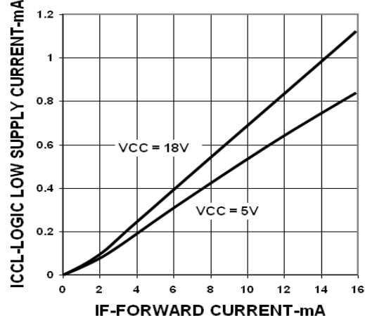
Figure 10: Logic LOW Supply Current vs. Forward Current
