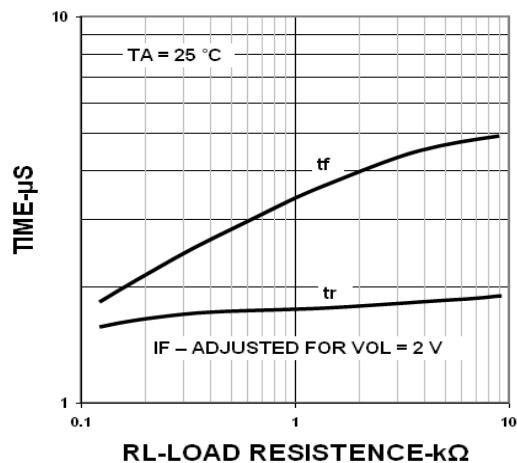
Figure 9: Non-Saturated Rise & Fall Times vs. Load Resistance
