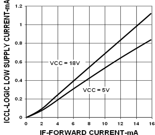
Figure 10: Logic LOW Supply Current vs. Forward Current
