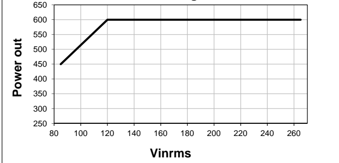
Line Derating
