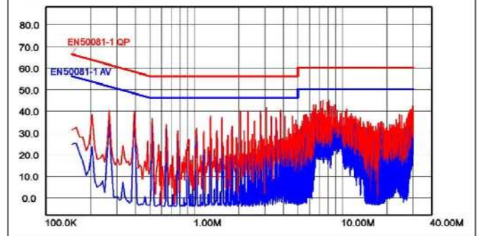
Typical Conducted Emmissions
