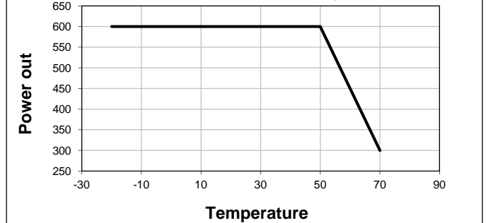
Temperature Derating
