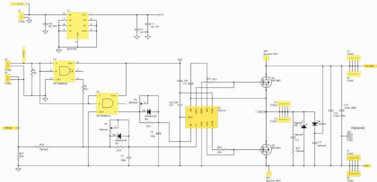
100 V Half-Bridge with Gate Drive, using EPC2007 Rev 2.0
