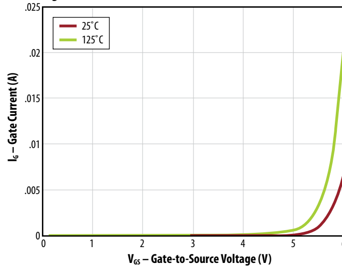
Figure 10: Gate Current
