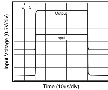
Figure 3: Overdrive Recovery
