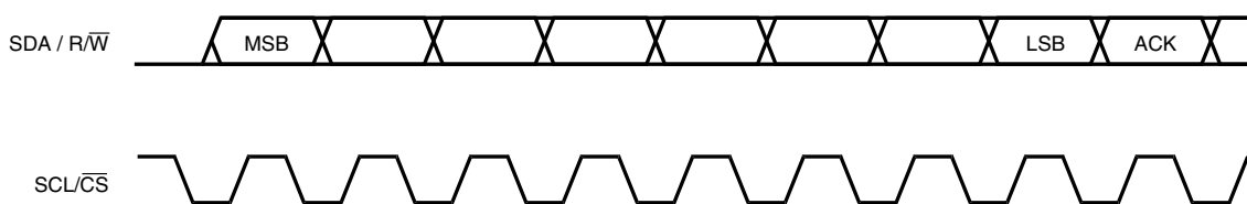
Figure 16. Serial Interface – Typical Byte Transfer
