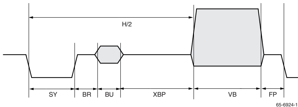
Figure 11. Horizontal Timing – 1st Half-line
