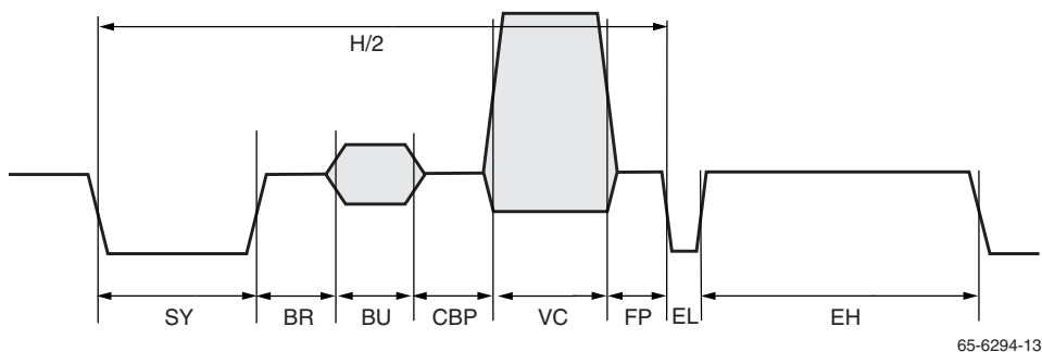
Figure 12. Horizontal Timing – 2nd Half-line
