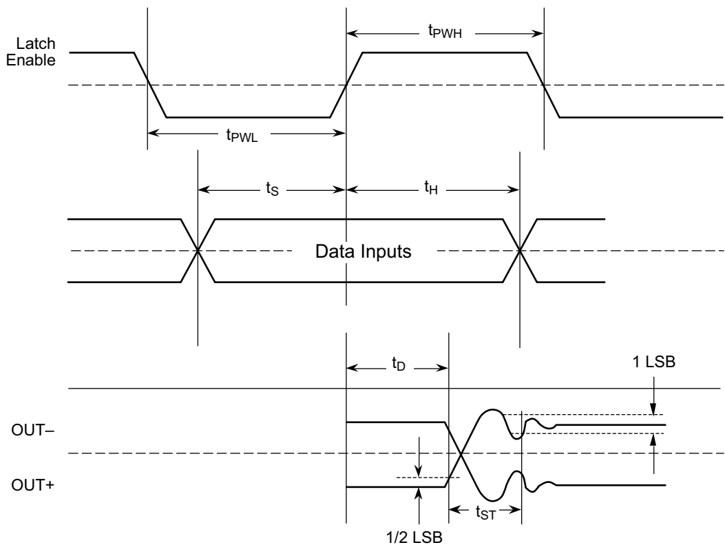
Figure 1 – Timing Diagram
