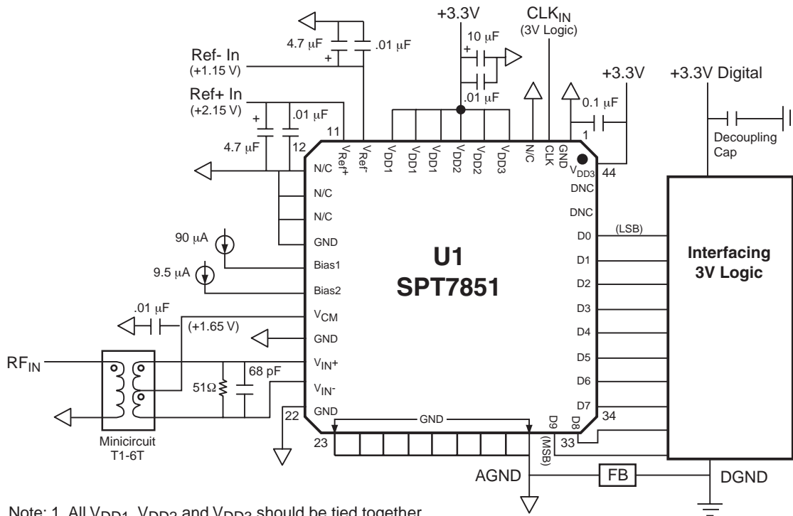
Figure 2: Typical Interface Circuit
