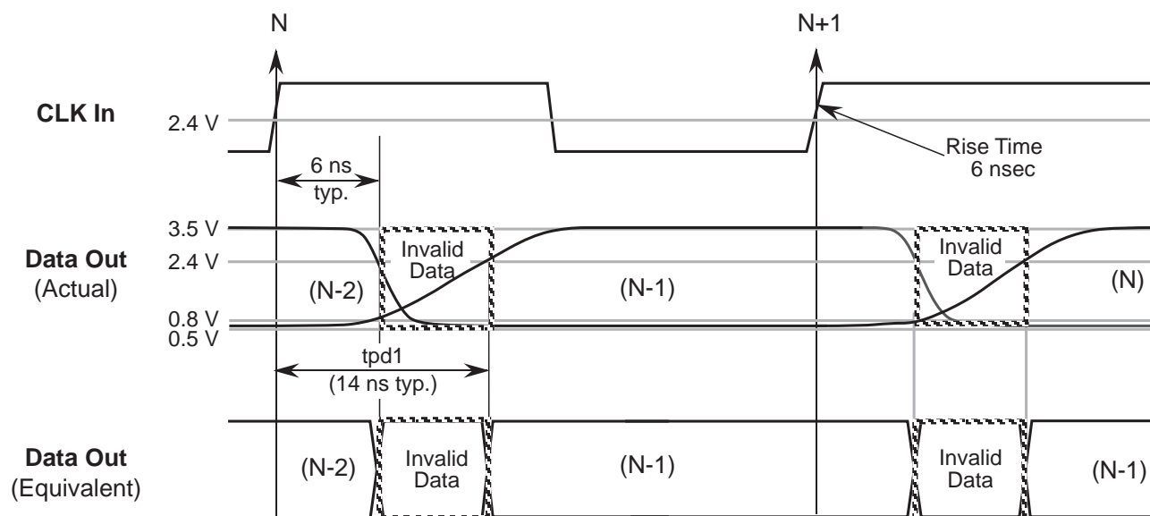
Figure 4 - Digital Output Characteristics
