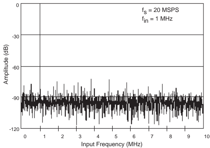
Spectral Response
