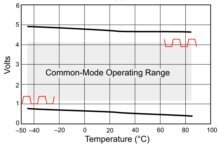
Differential Input Common-Mode Operating Range 400 mV P-P
