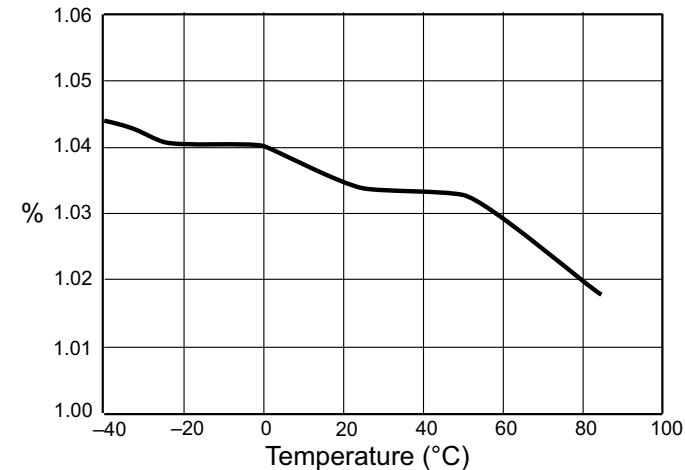
Percent Gain Error vs Temperature
