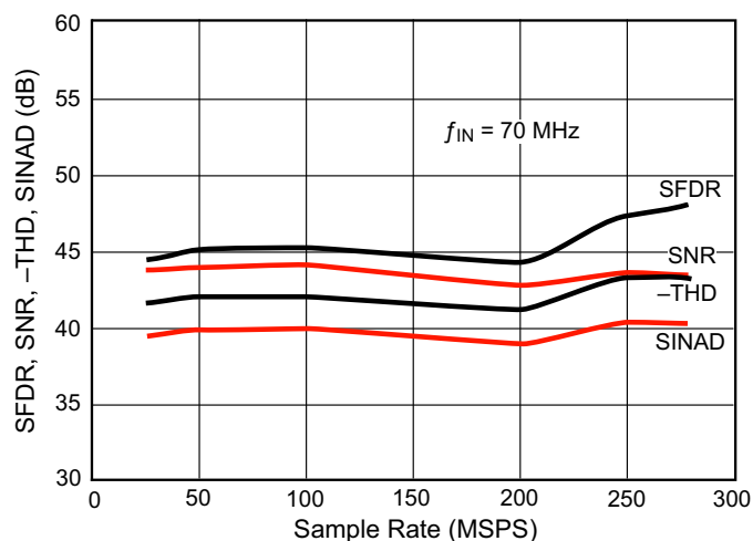
AC Performance vs Sample Rate
