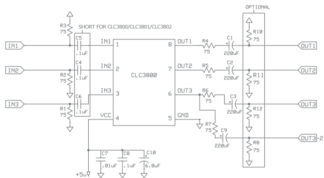
Figure 9. CEB021 Schematic
