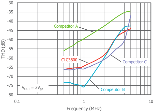
Total Harmonic Distortion DC-Coupled Out (R L = 75Ω)
