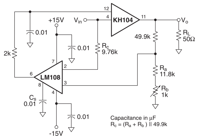
Figure 2: Composite Amplifier
