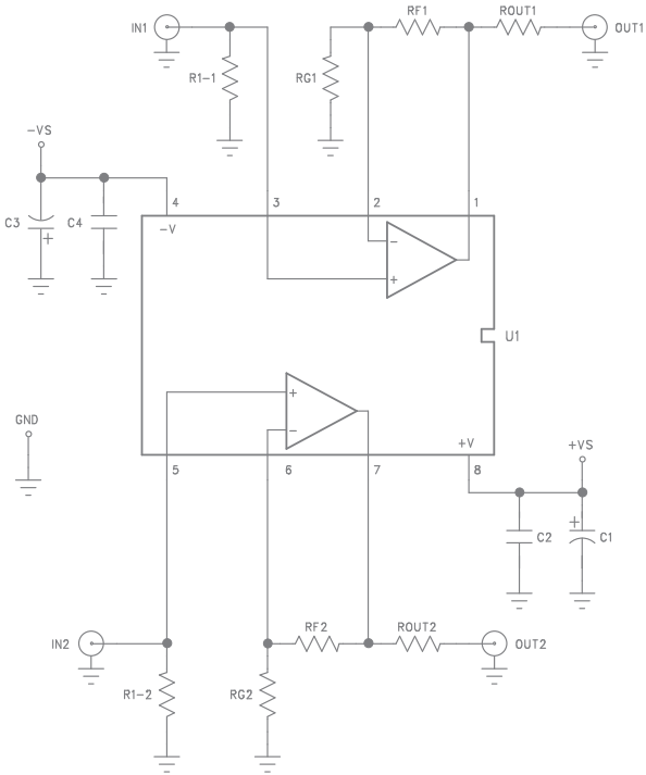
Figure 9. CEB006 Schematic
