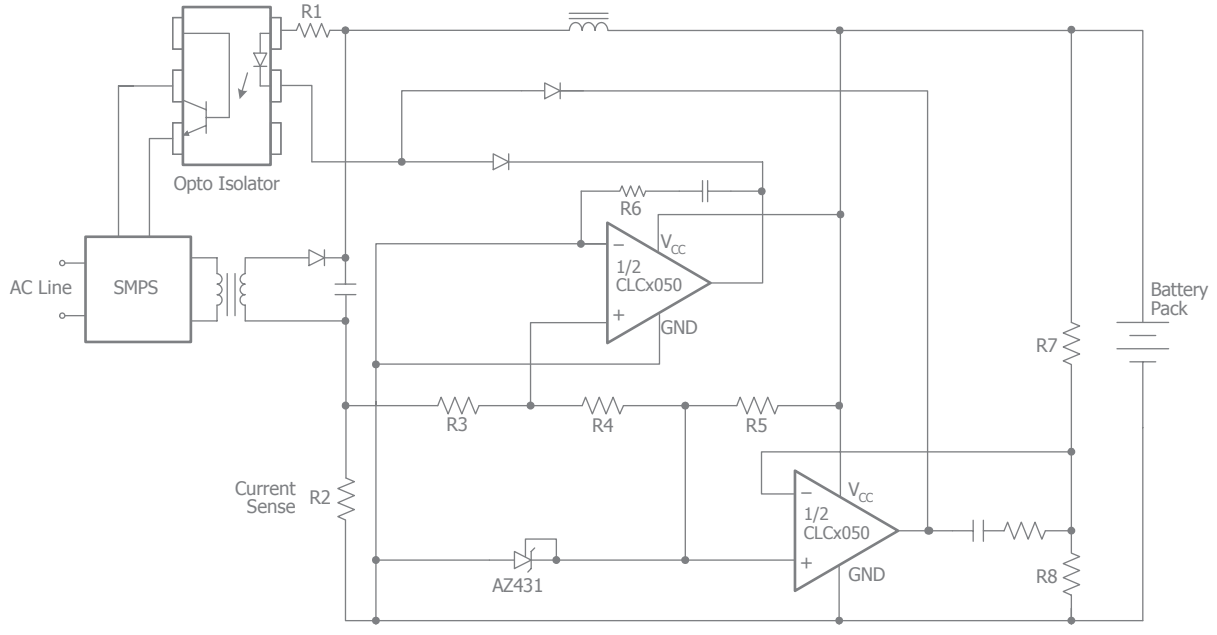
Figure 16. Battery Charger
