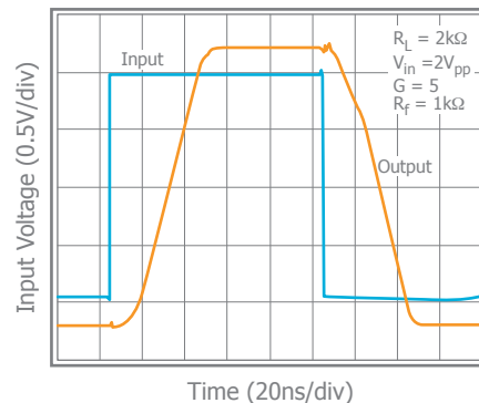
Figure 9. Overdrive Recovery
