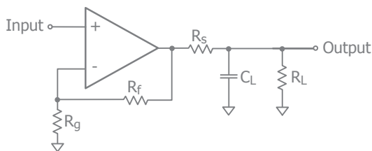
Figure 8. Addition of R_S for Driving Capacitive Loads
