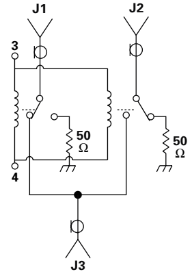
-1 (FAILSAFE)
