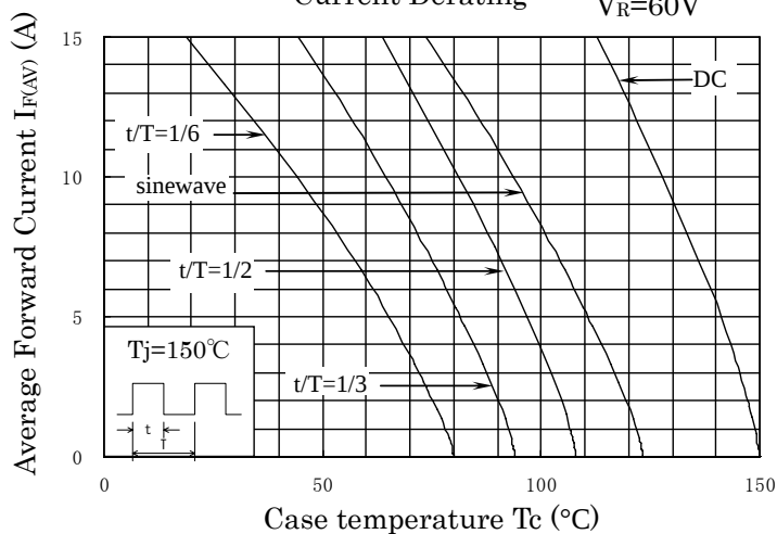
Current Derating
