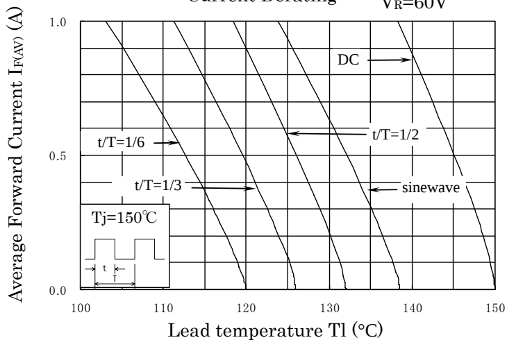
Current Derating
