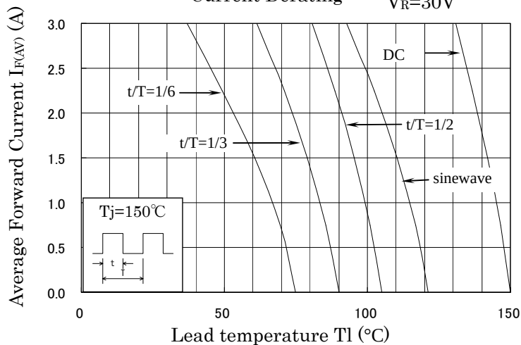
Current Derating
