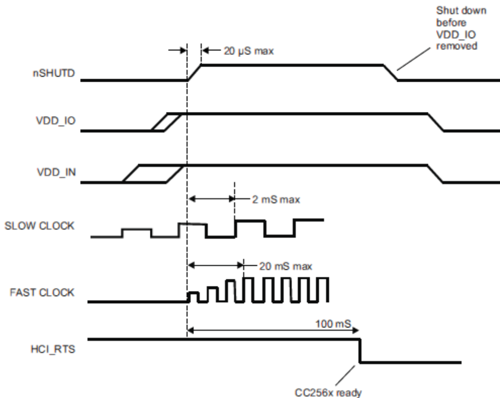
Figure 11 Power-up sequence
