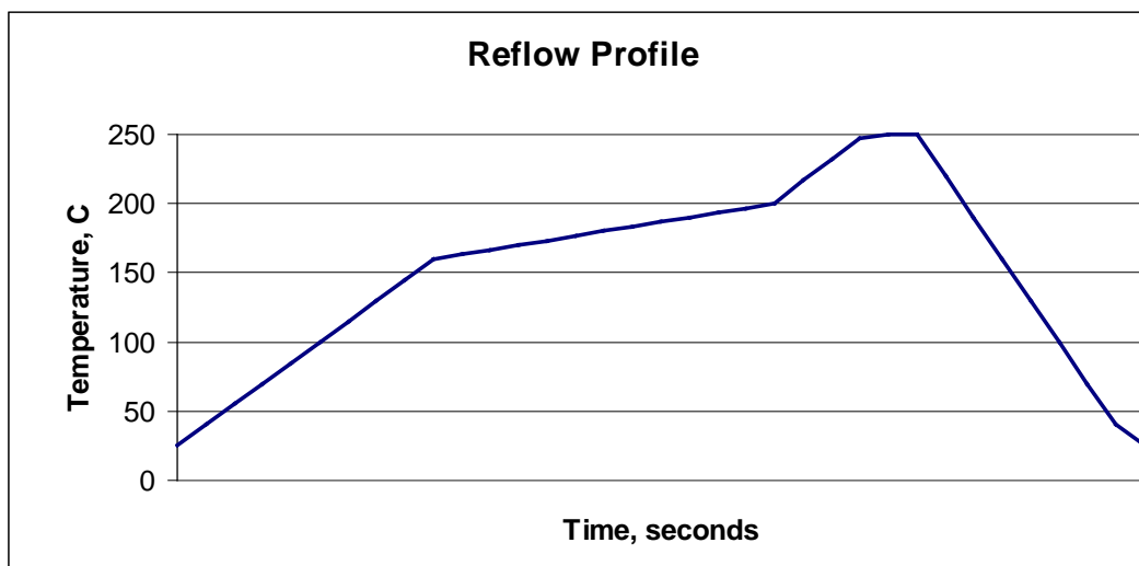
Figure 12 Reflow Profile Pattern
