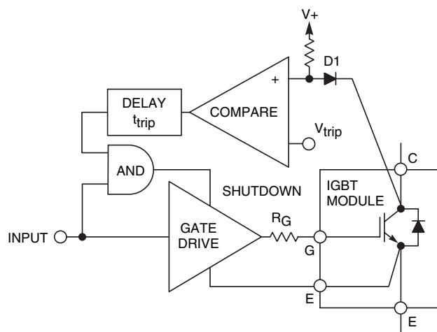
Figure 1. Desaturation Detector
