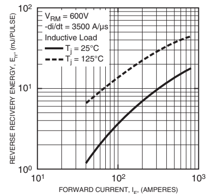
REVERSE RECOVERY ENERGY CHARACTERISTICS (TYPICAL)
