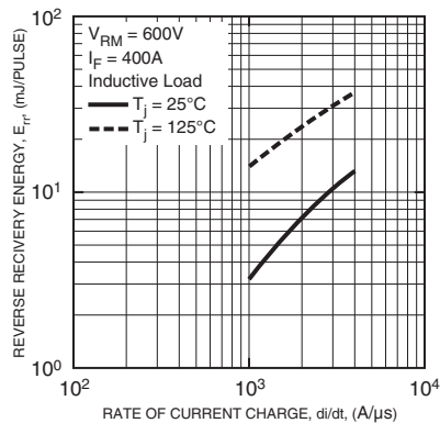
REVERSE RECOVERY ENERGY CHARACTERISTICS (TYPICAL)
