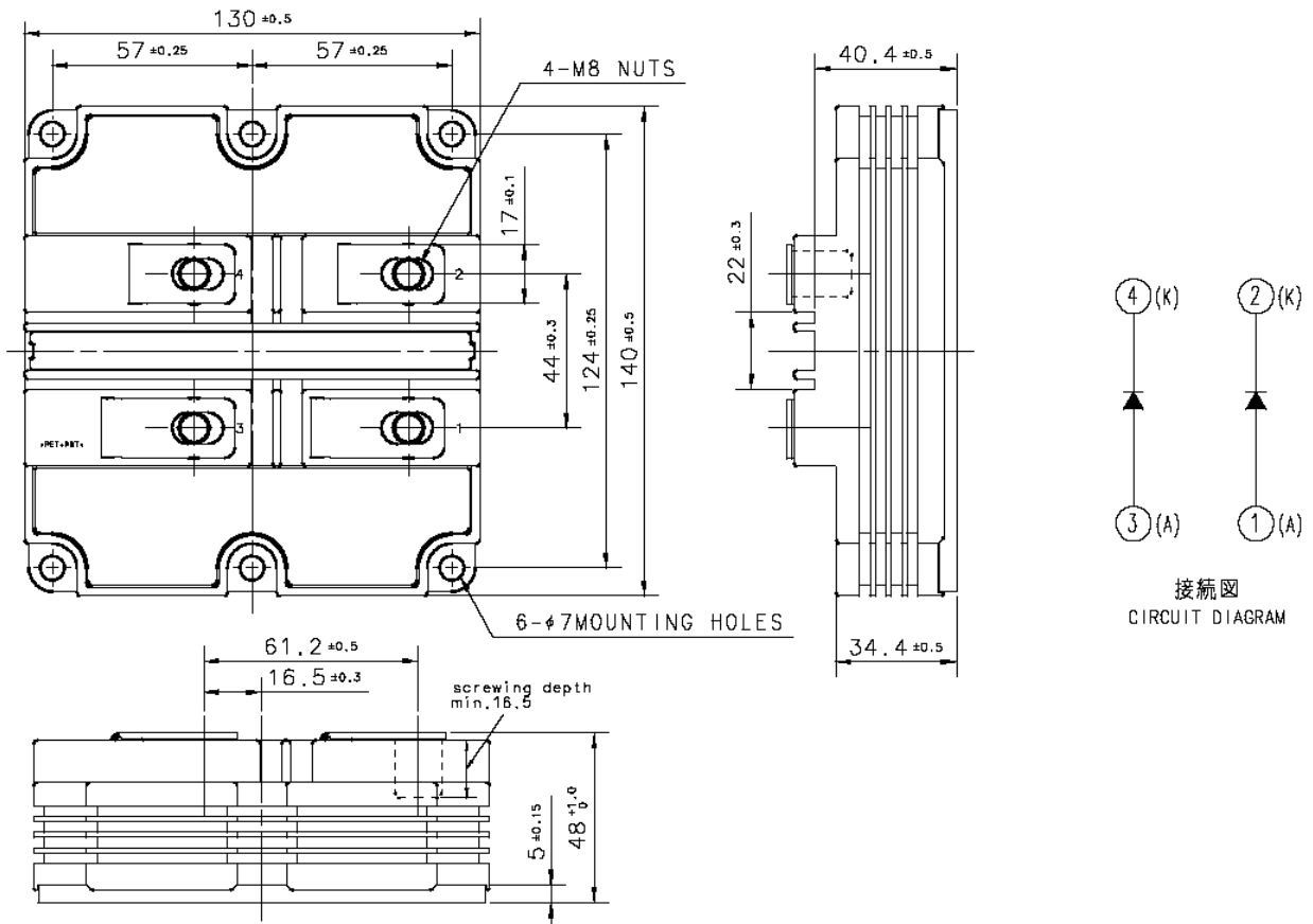
Fig. 1 - Outline drawing
