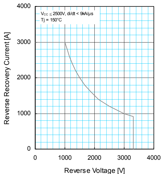
REVERSE RECOVERY SAFE OPERATING AREA (TYPICAL)
