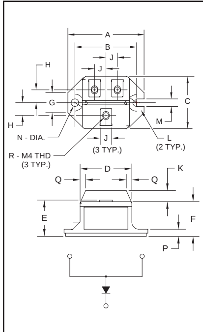
Outline Drawing
