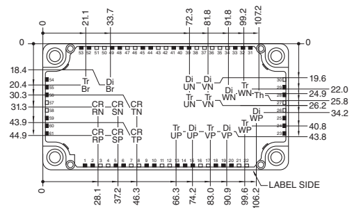
Each mark points to the center position of each chip. Tr^*P / Tr^*N / Tr^*Br (* = U/V/W); IGBT Di^*P / Di^*N (* = U/V/W); FWDi DiBr: Clamp Di CR^*P / CR^*N (* = R/S/T); Conv Di Th: NTC Thermistor
