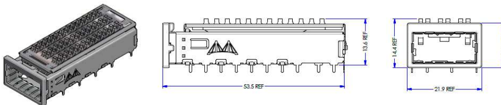
Figure 1. MA000603 Mechanical Drawings and Information
