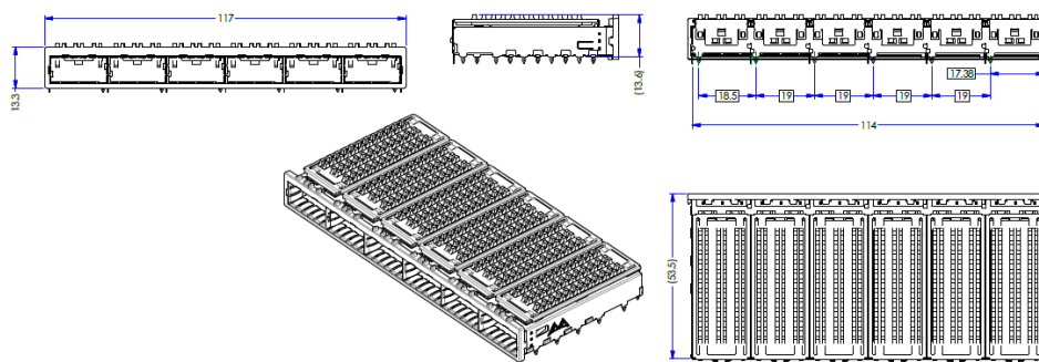
Figure 3. MA000598 Mechanical Drawings and Information
