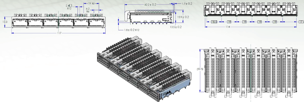
Figure 2. MA000597 Mechanical Drawings and Information
