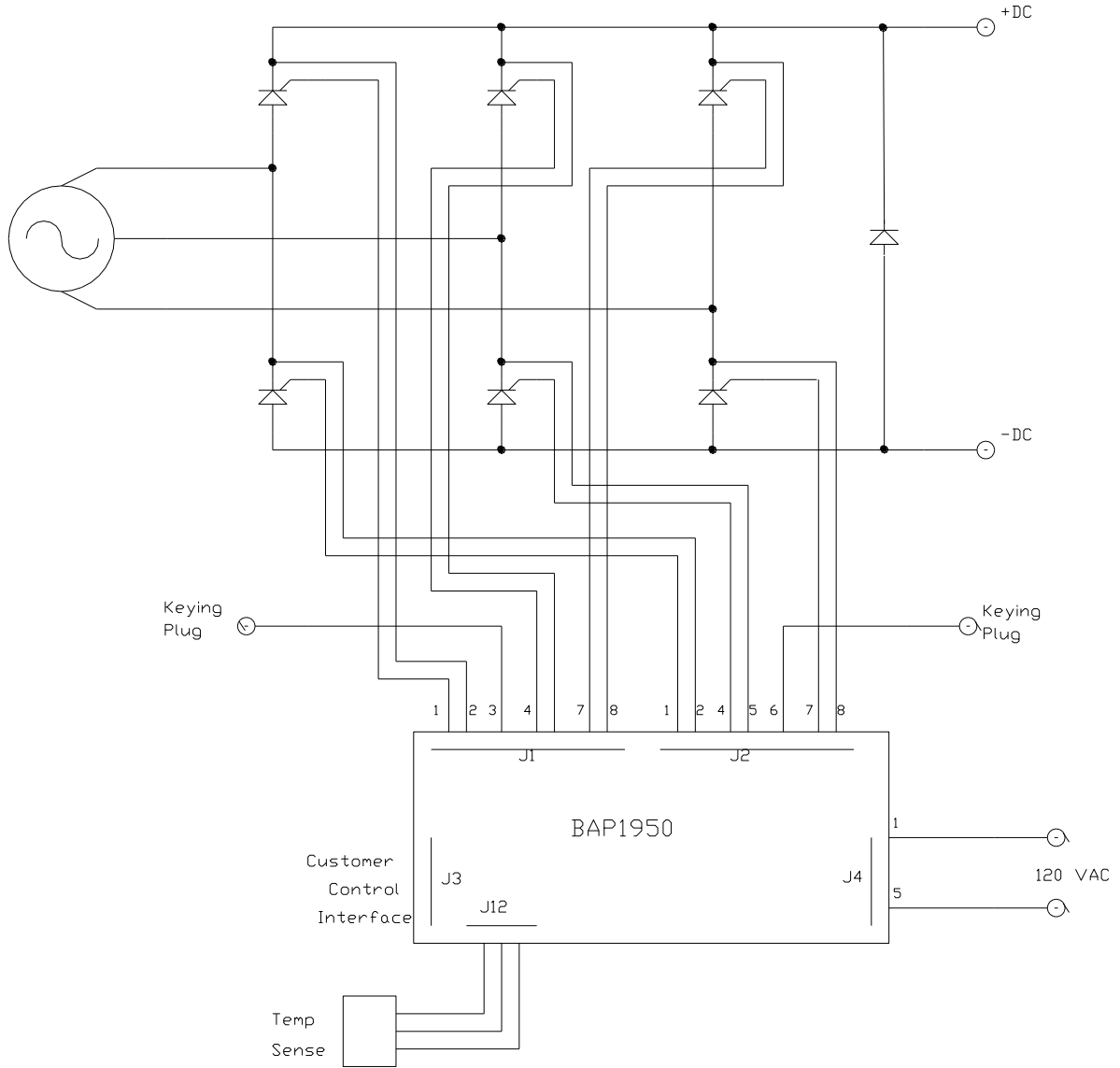
Schematic of AC-DC Open Loop Converter
