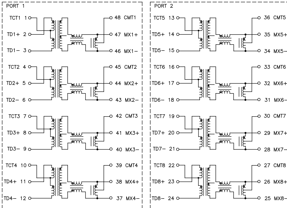
SCHEMATIC
