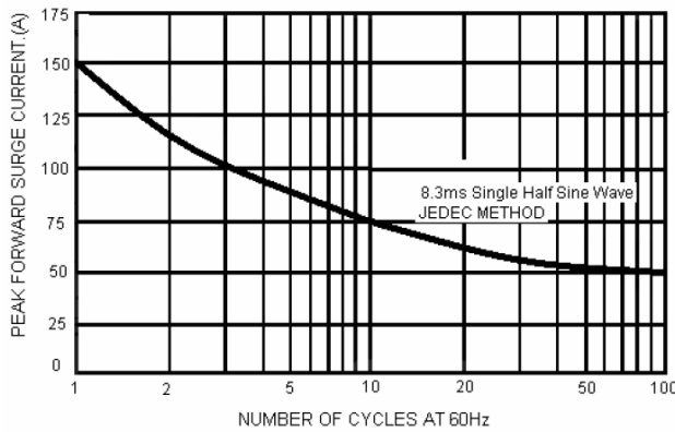
FIG.1-MAXIMUM NONO-REPETITIVE FORWARD SURGE CURRENT PER BRIDGE ELEMEN
