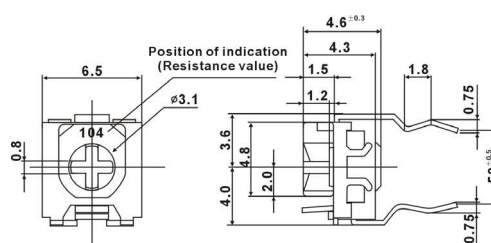
TSR-3318F FRONT VIEW
