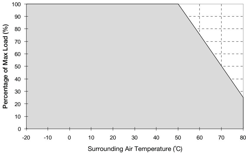
Fig. 1.1 De-rating for Vertical Mounting Orientation > 50°C de-rate power by 2.5% / °C, > 70°C to 75°C de-rate power by 5% / °C
