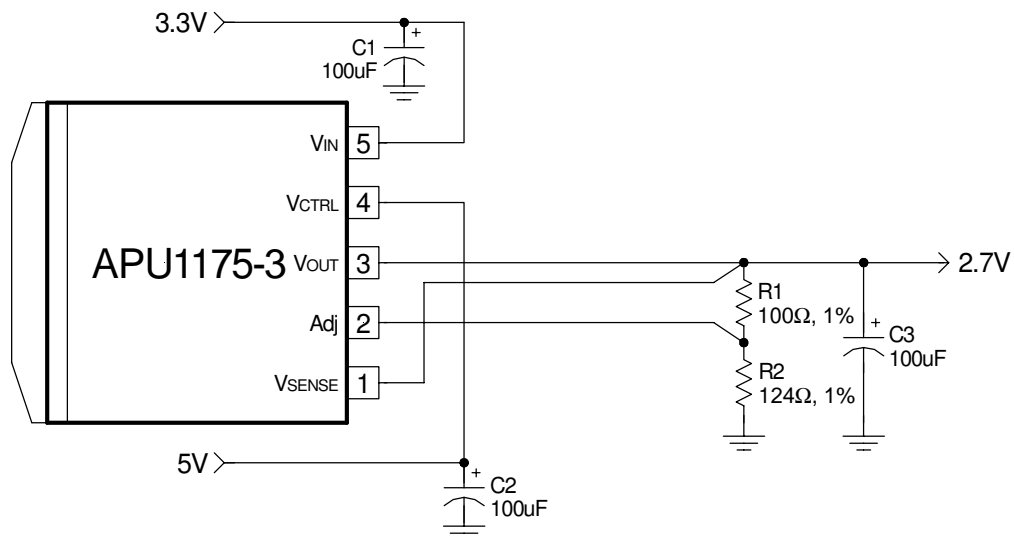
Figure 1 - Typical application of APU1175 in a 3.3V to 2.7V supply.
