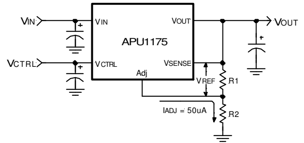
Figure 3 - Typical application of the APU1175 for programming the output voltage.
