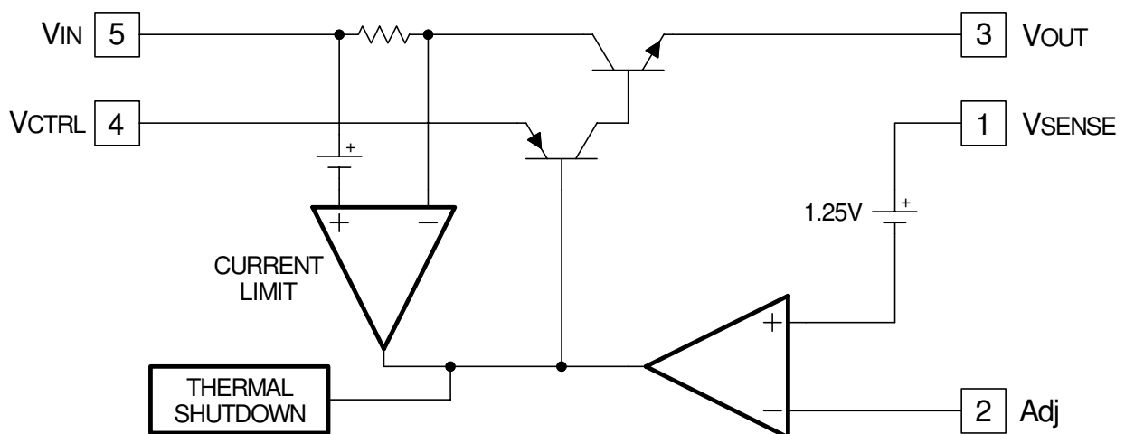
Figure 2 - Simplified block diagram of the APU1175.
