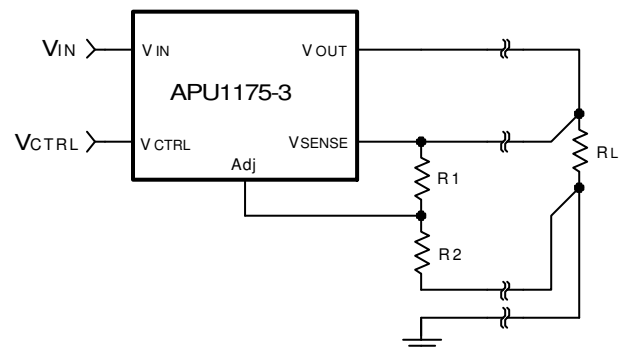
Figure 4 - Schematic showing connection for best load regulation.
