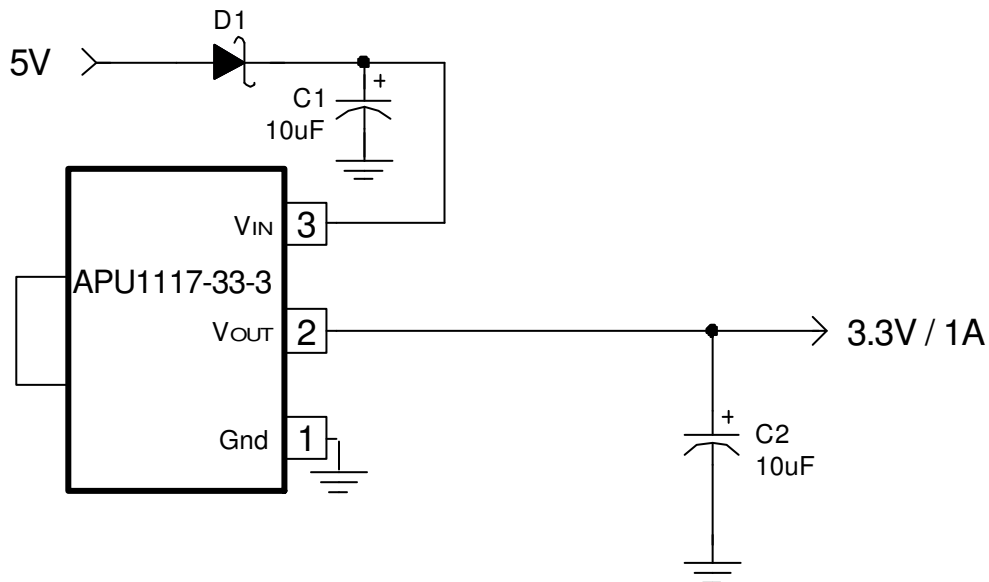
Figure 1 - Typical application of APU1117-33-3 in a 5V to 3.3V regulator.
