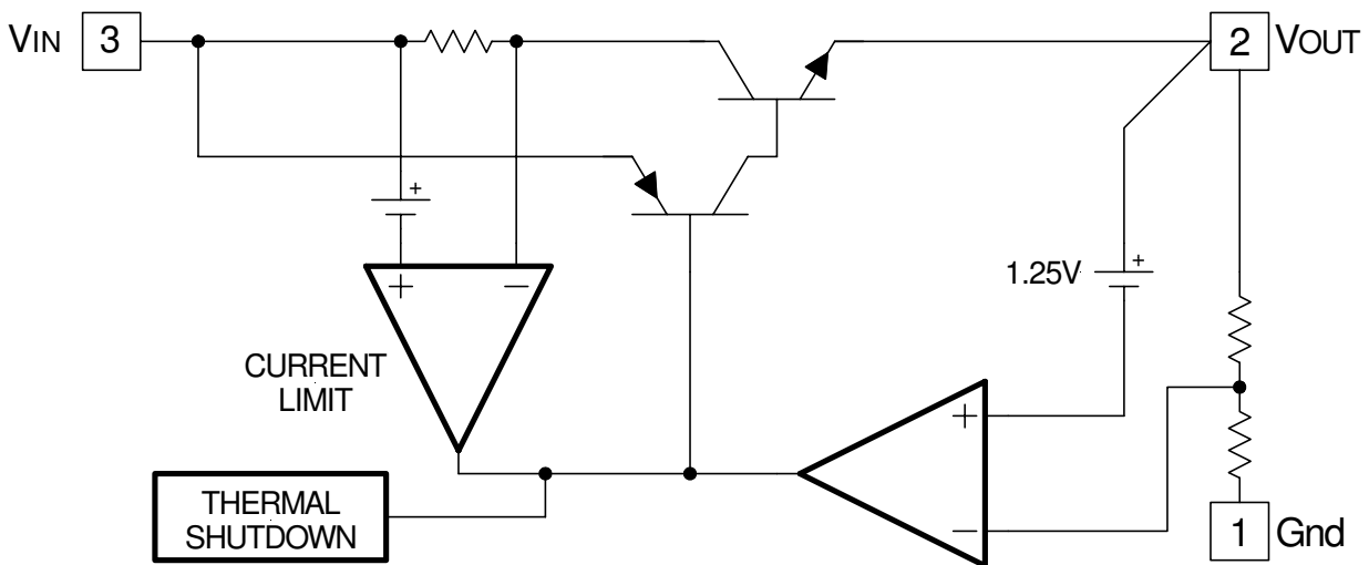
Figure 2 - Simplified block diagram of the APU1117-33-3.
