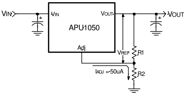
Figure 3 - Typical application of the APU1050 for programming the output voltage.
