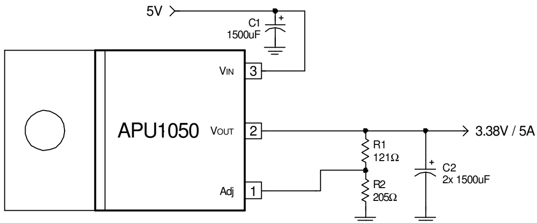
Figure 1 - Typical Application of APU1050 in a 5V to 3.38V regulator
