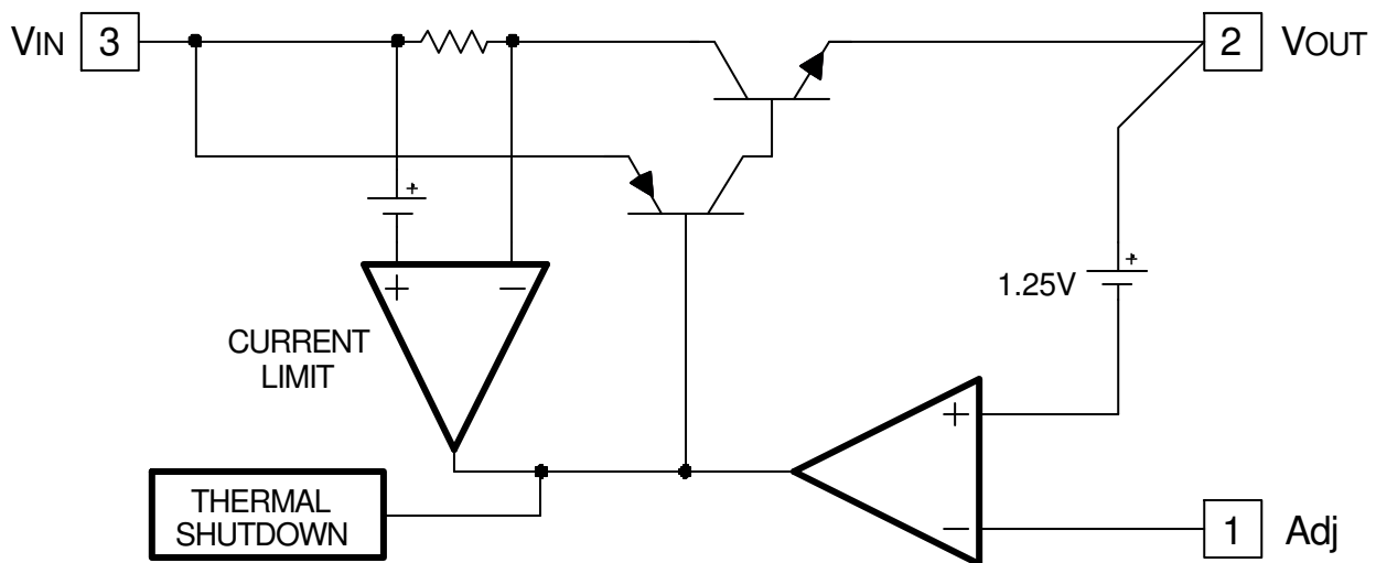
Figure 2 - Simplified block diagram of the APU1050.
