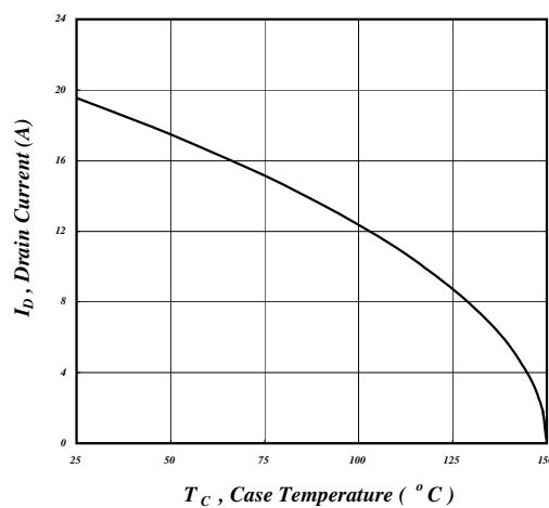
Fig 12. Maximum Continuous Drain Current vs. Junction Temperature
