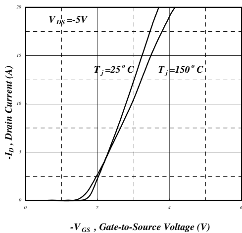
Fig 11. Transfer Characteristics
