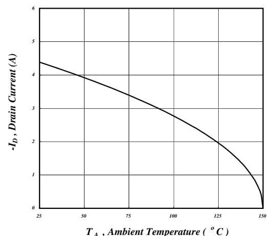
Fig 12. Maximum Continuous Drain Current vs. Ambient Temperature
