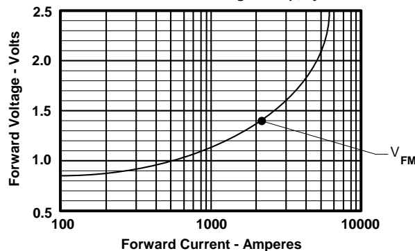
Maximum Forward Voltage Drop, T J 180 C
