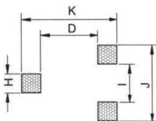
LAND PATTERN
