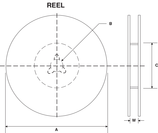
REEL DIMENSIONS (mm)
