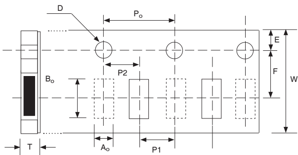
CARDBOARD CARRIER TAPE
