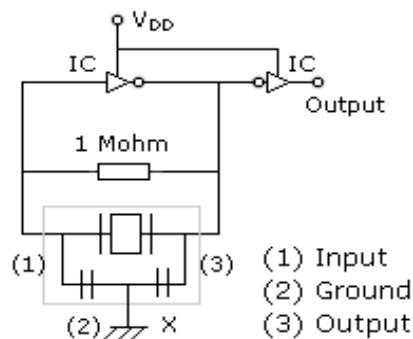
Test Circuit
