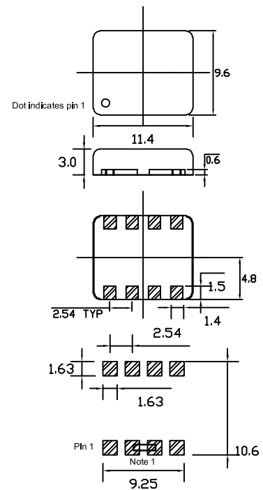
Recommended solder pad layout Note 1: Connect pin 2 to pin 3
