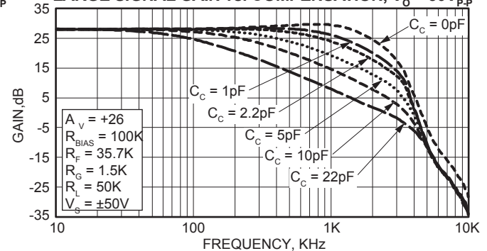
LARGE SIGNAL GAIN vs. COMPENSATION, V_O = 50\text{V}_{P-P}
